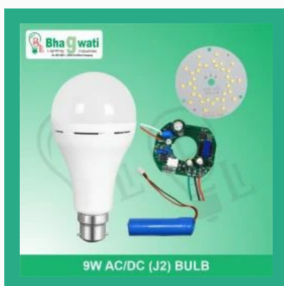
9W ACDC Rechargeable Bulb (2000 Mah with PBT) JADU2
